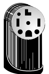
Figure 2 4-wire receptacle (14-30R)
